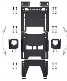
SIDEMT001A Side Mount (Universal)
