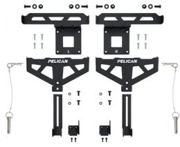
XBEDMT001C Cross-Bed Mount (Ford BoxLink)
