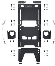
SIDE MT001B Side Mount (Toyota Deck Rail)
