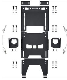
SIDE MT001A Side Mount (Universal)
